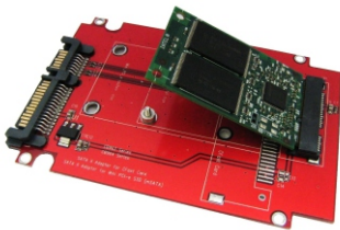
full size mSATA
